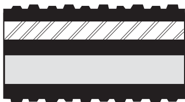
STYLE A - STEEL PLATE BONDED BETWEEN NRC AND FLATBACK PADS
