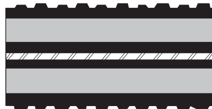
STYLE E - GALVANIZED STEEL PLATE BONDED BETWEEN MULTIPLE NRC PADS
